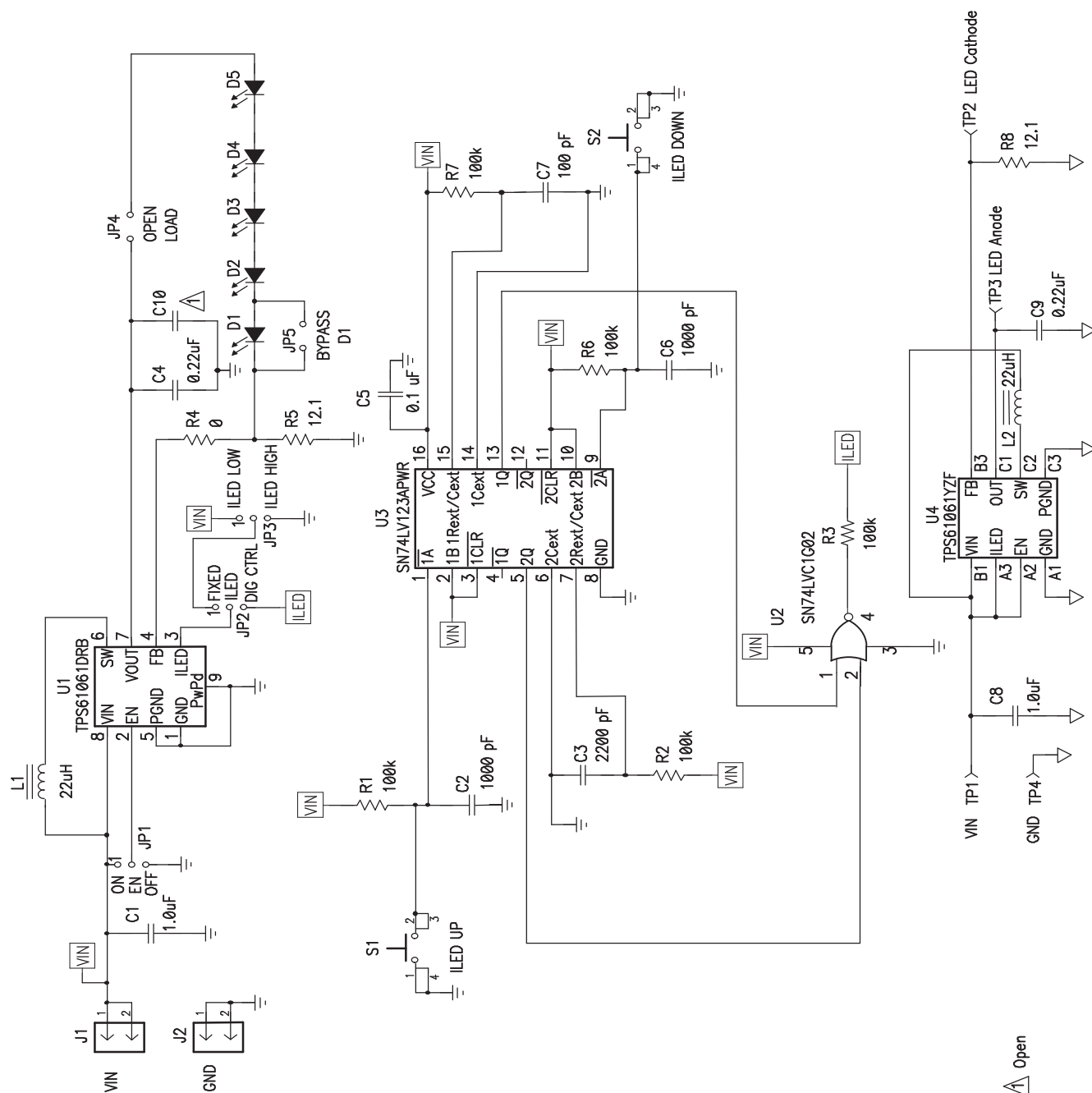
Figure 4. TPS6106xEVM Schematic
